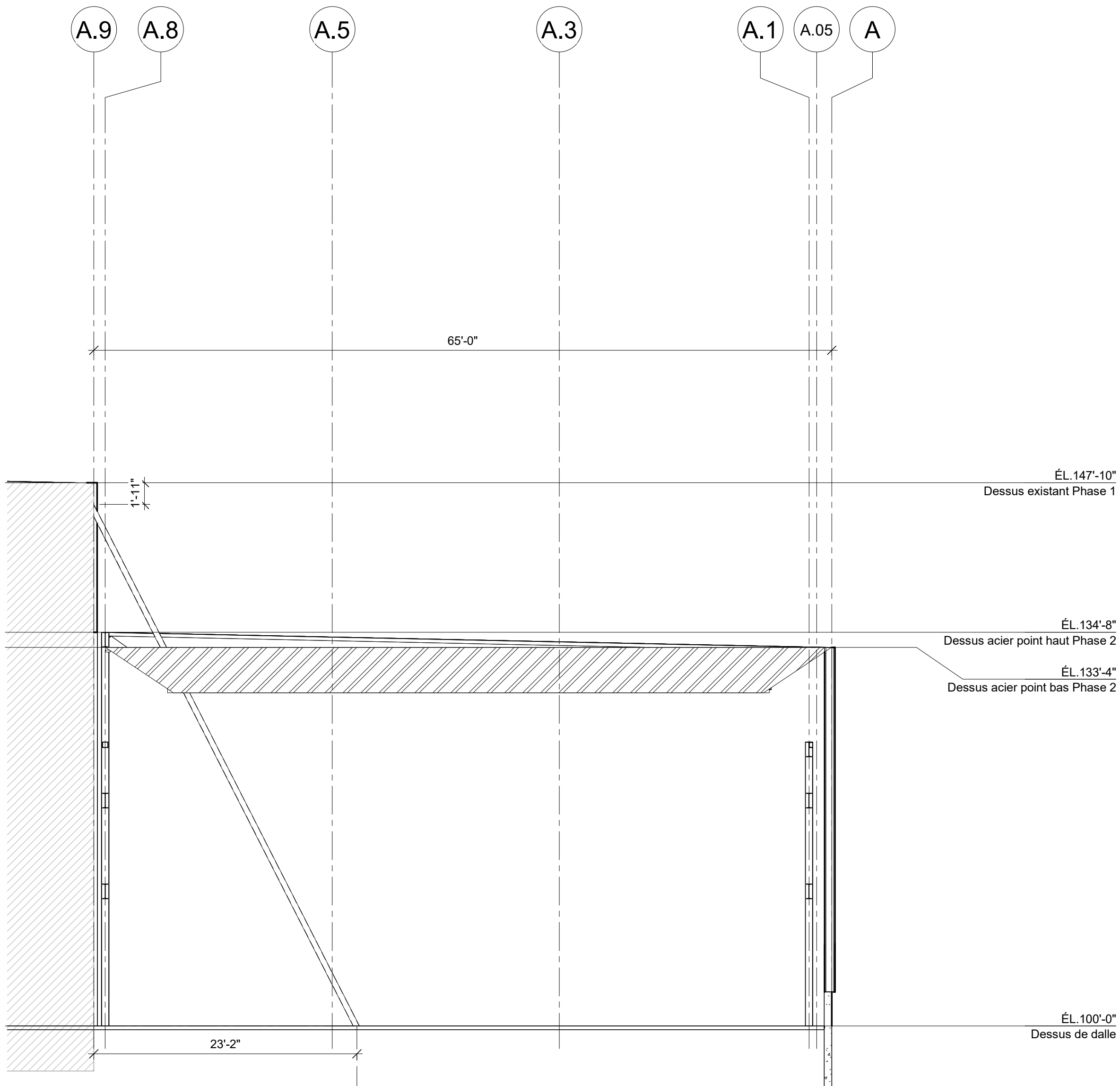
AXE 10.9 (STRUCTURE) 1/8" = 1'-0"
