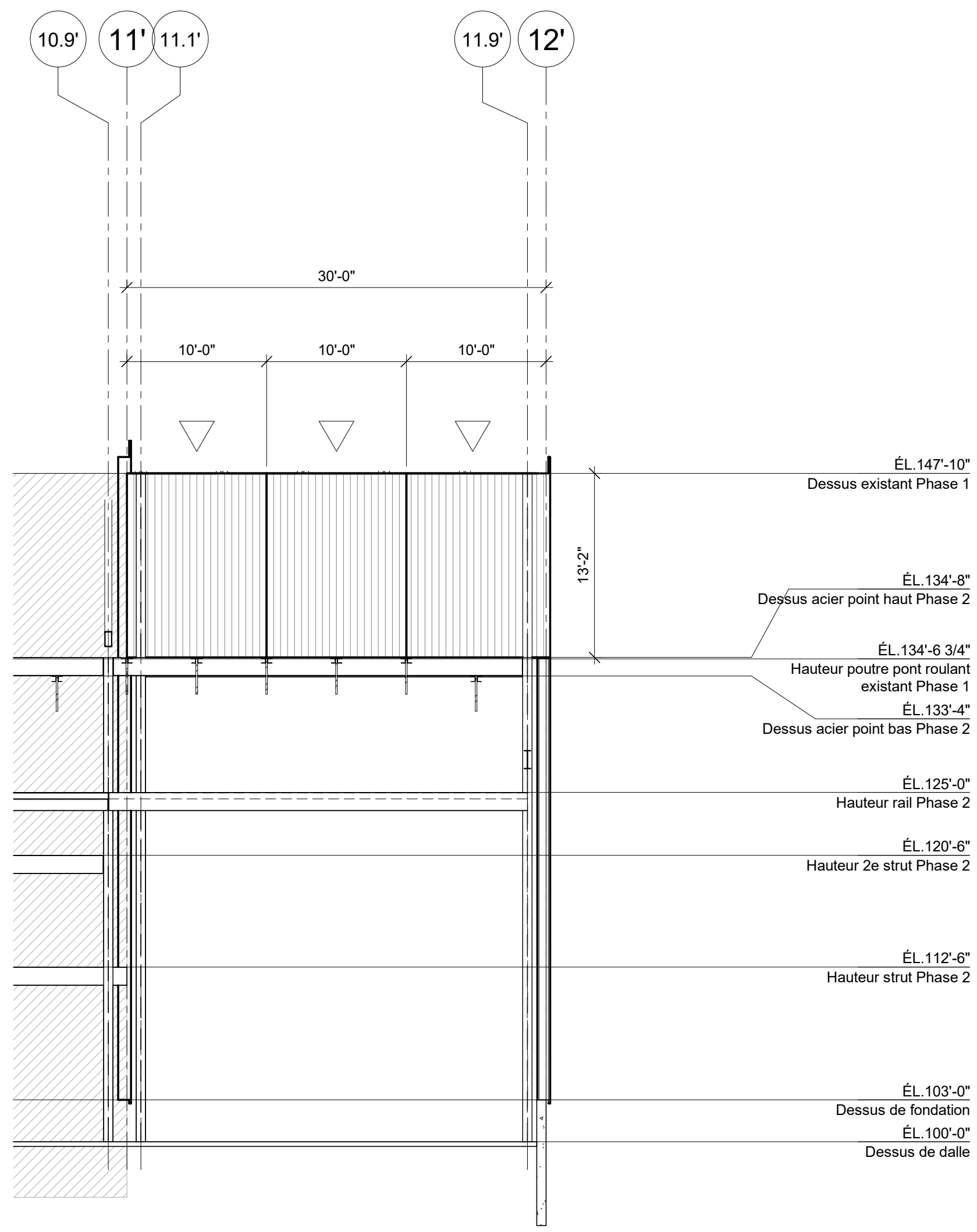
AXE A.9 (high & low) 1/8" = 1'-0"
