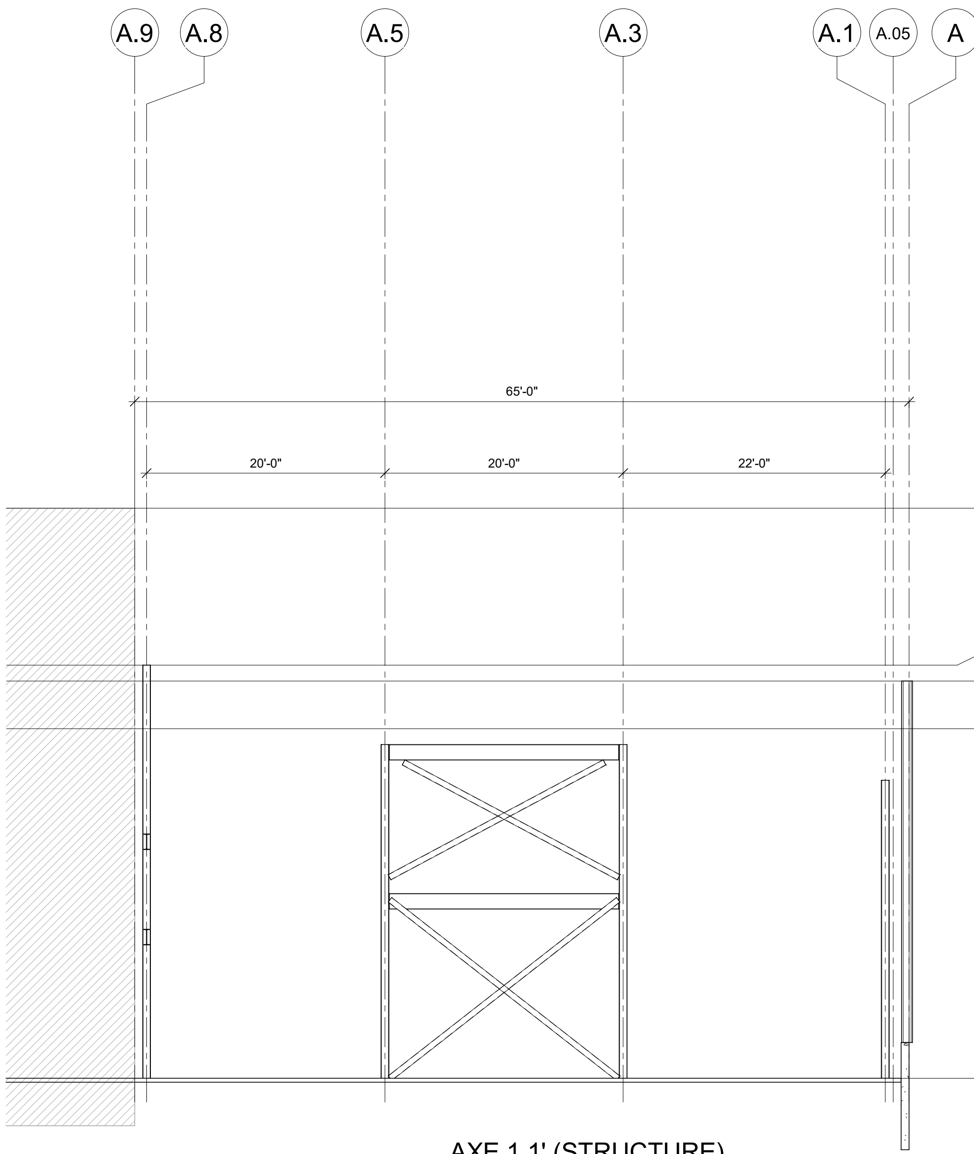
AXE 1.1' (STRUCTURE) 1/8" = 1'-0"
